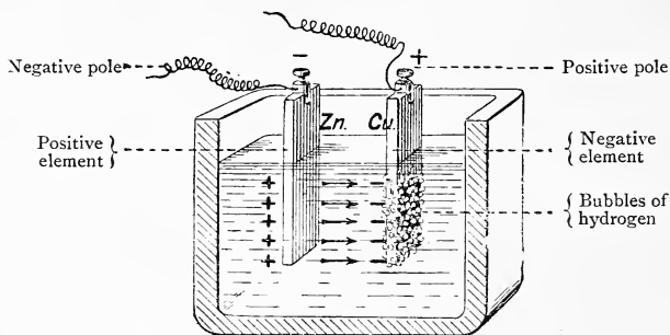
FIG. 1.—GALVANIC CELL.
